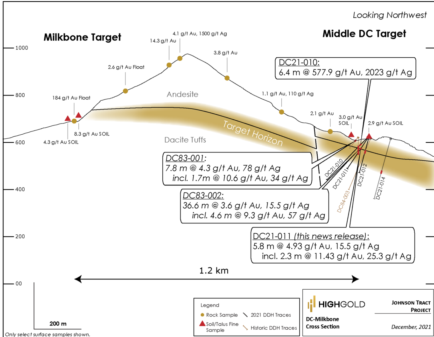
Figure 2. Johnson Tract Project – DC Prospect Schematic Cross-Section from Middle DC to Milkbone
