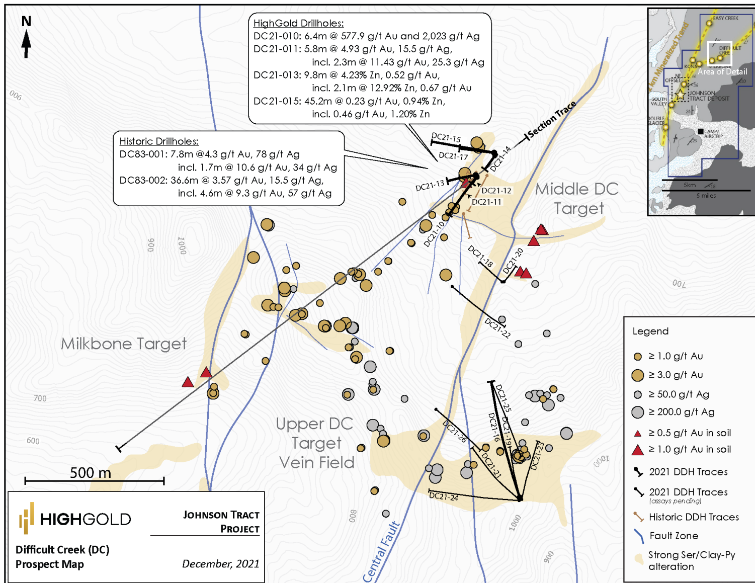
Figure 1. Johnson Tract Project – DC Prospect 2021 Drill Hole Plan Map (4km Northeast of JT Deposit)
